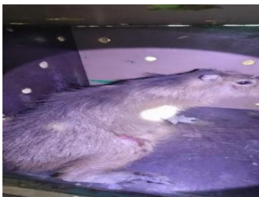
(58040) Capivara
