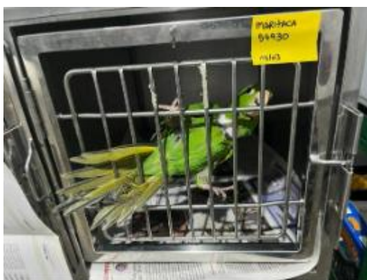
(54930) Maritaca
